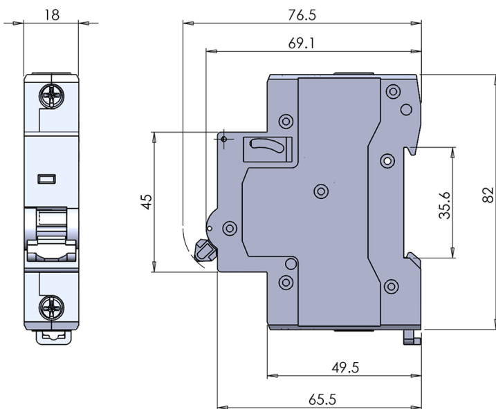
Line Drawing - PBM32B
