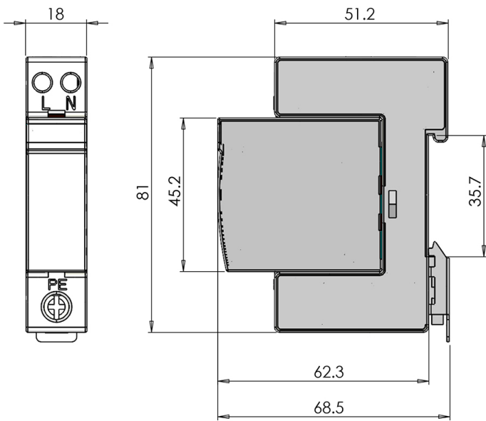
Line Drawing - PBSPD
