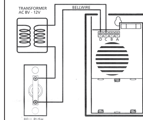
Circuit Diagram with Illuminating bell push
