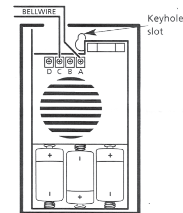
Circuit Diagram for normal bell push
